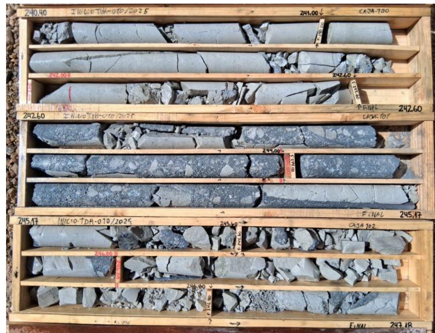
Diatreme breccia with sulphide matrix at the end of hole TDH-010
